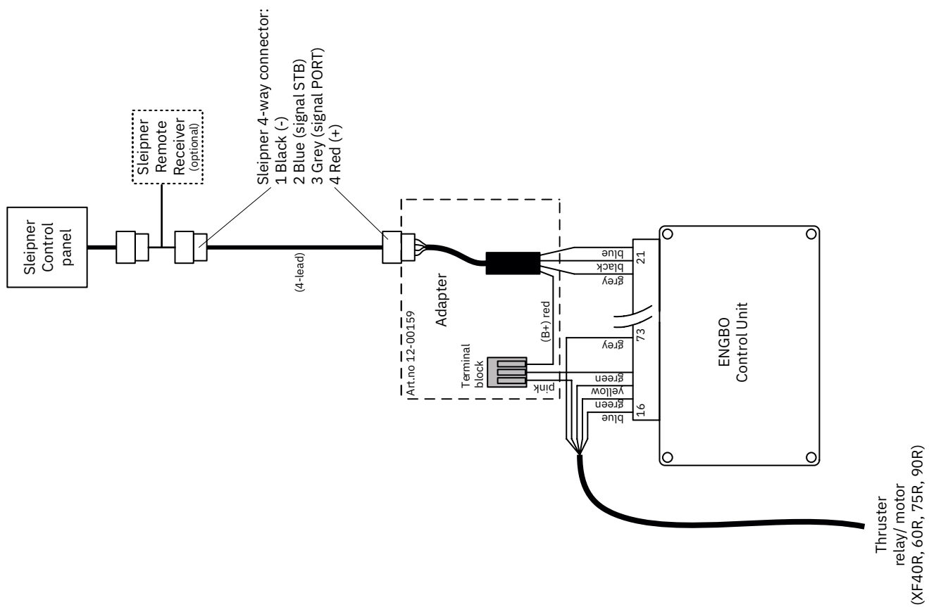
Connection of ENGBO thruster / Sleipner panel - adapter (art.no 12-00159)
